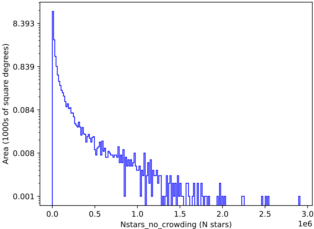
too_10_4v3.4_10yrs u: Nstars_no_crowding
