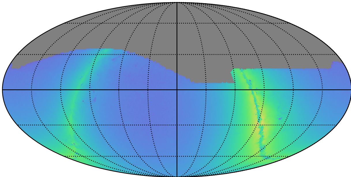
too_10_4v3.4_10yrs r: Nstars_no_crowding
