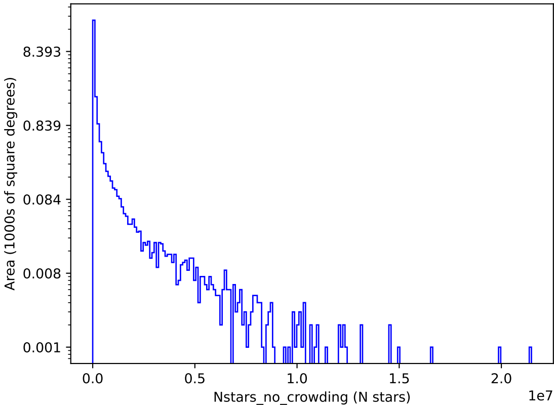
too_10_4v3.4_10yrs r: Nstars_no_crowding
