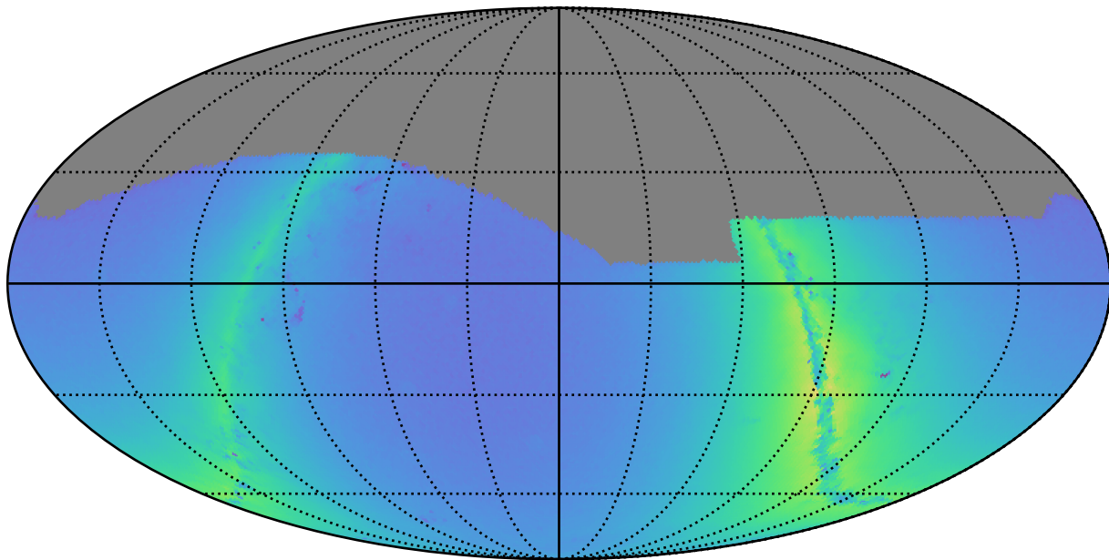
too_10_4v3.4_10yrs g: Nstars_no_crowding
