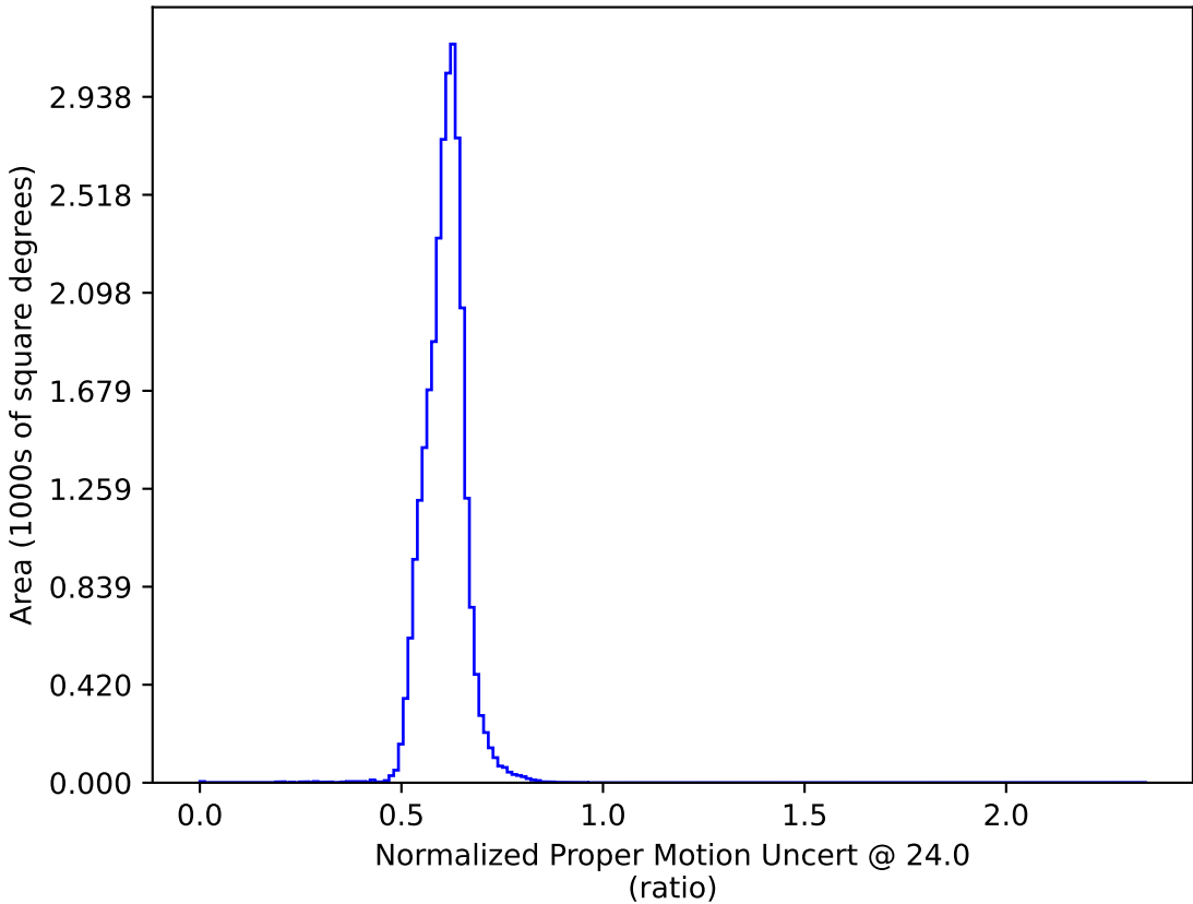
too_10_4v3.4_10yrs : Normalized Proper Motion Uncert @ 24.0
