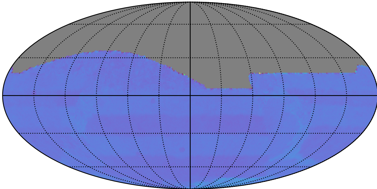
too_10_4v3.4_10yrs : Normalized Proper Motion Uncert @ 20.5
