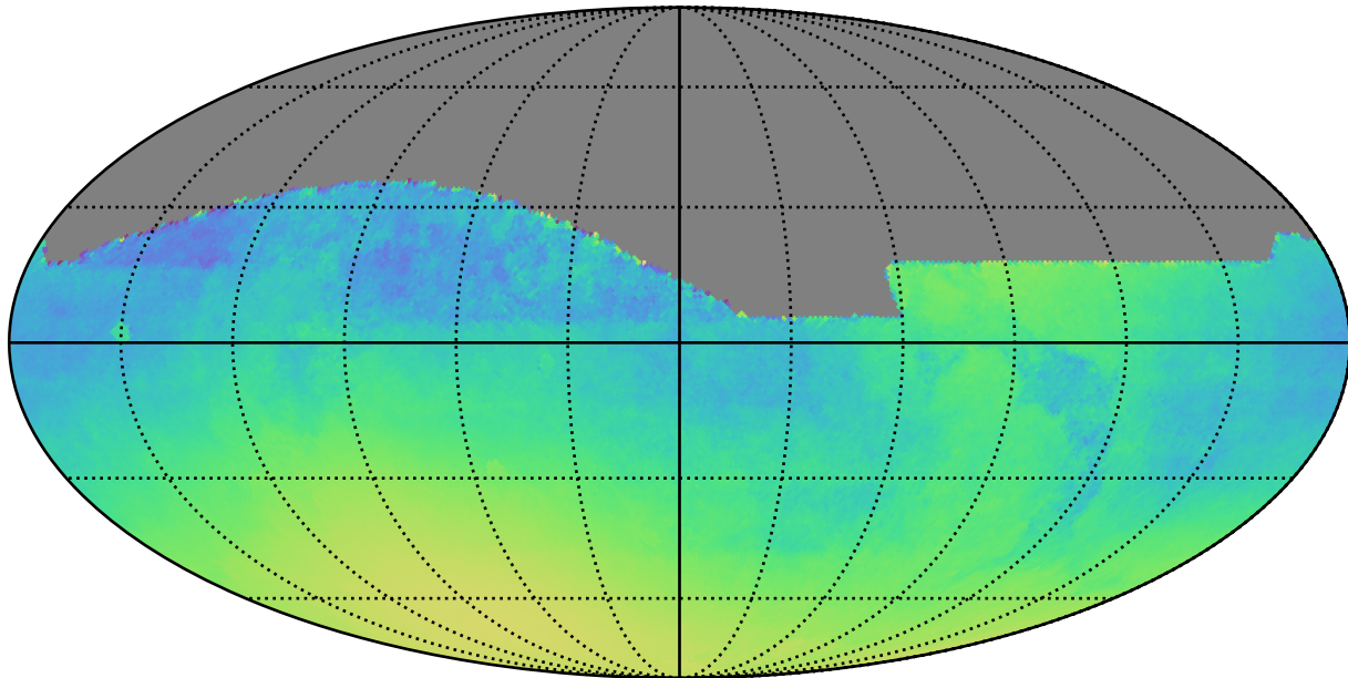
too_10_4v3.4_10yrs : Normalized Parallax Uncert @ 24.0
