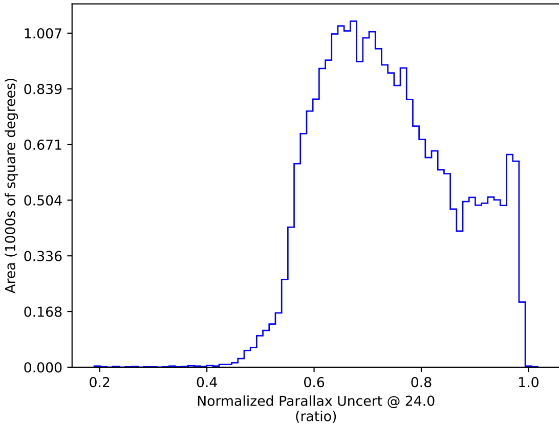
too_10_4v3.4_10yrs : Normalized Parallax Uncert @ 24.0
