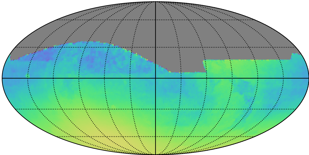
too_10_4v3.4_10yrs : Normalized Parallax Uncert @ 22.4
