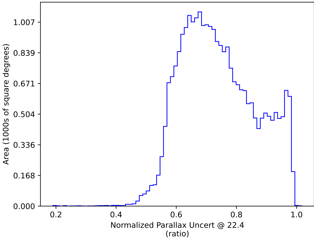
too_10_4v3.4_10yrs : Normalized Parallax Uncert @ 22.4
