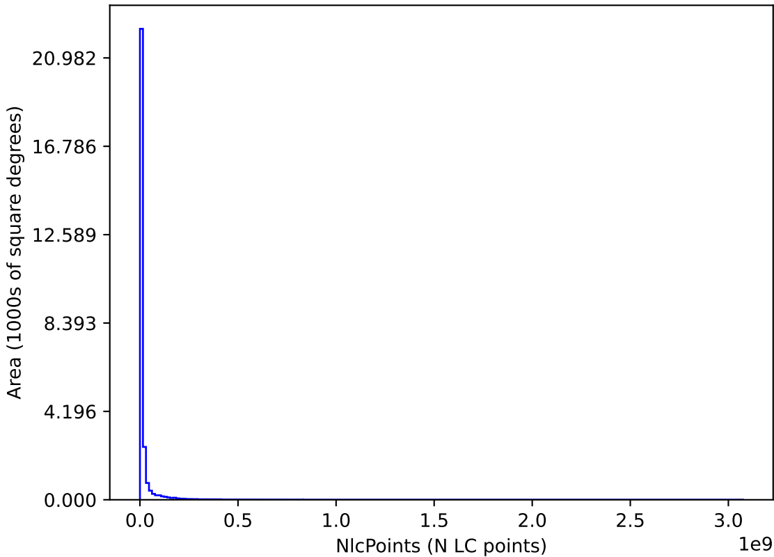
too_10_4v3.4_10yrs : NlcPoints
