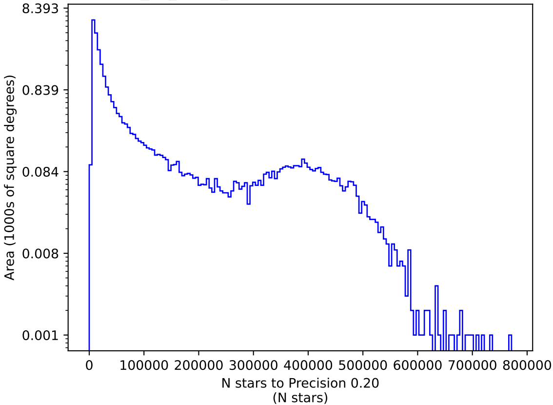
too_10_4v3.4_10yrs z: N stars to Precision 0.20
