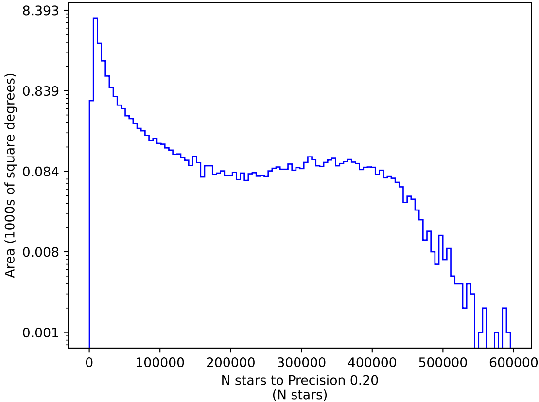
too_10_4v3.4_10yrs y: N stars to Precision 0.20
