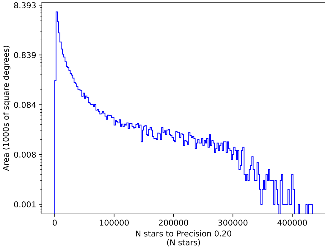
too_10_4v3.4_10yrs u: N stars to Precision 0.20
