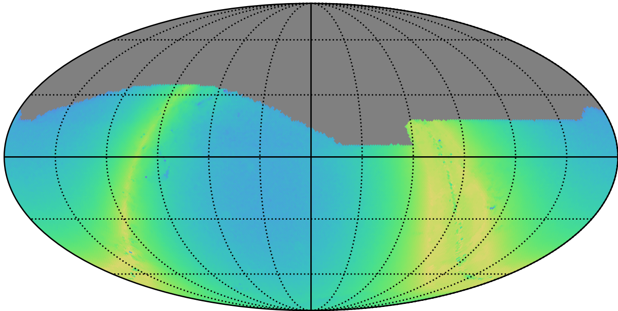
too_10_4v3.4_10yrs r: N stars to Precision 0.20
