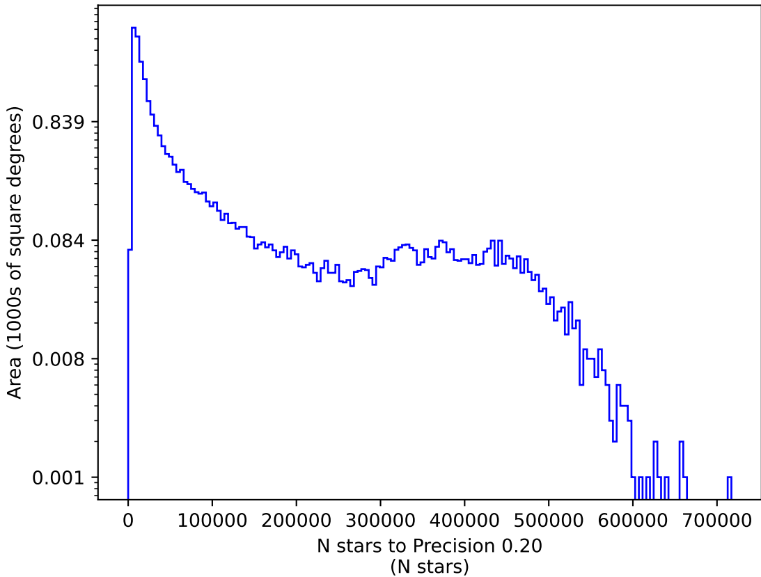
too_10_4v3.4_10yrs r: N stars to Precision 0.20
