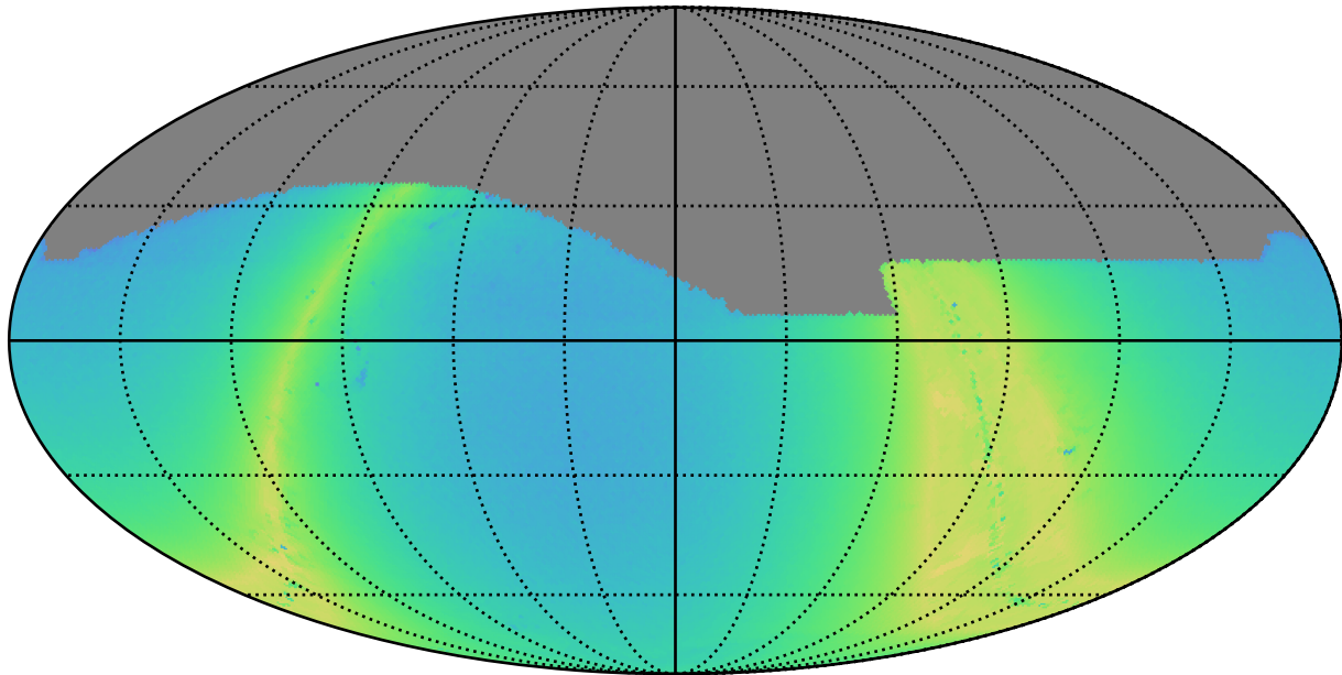
too_10_4v3.4_10yrs i: N stars to Precision 0.20
