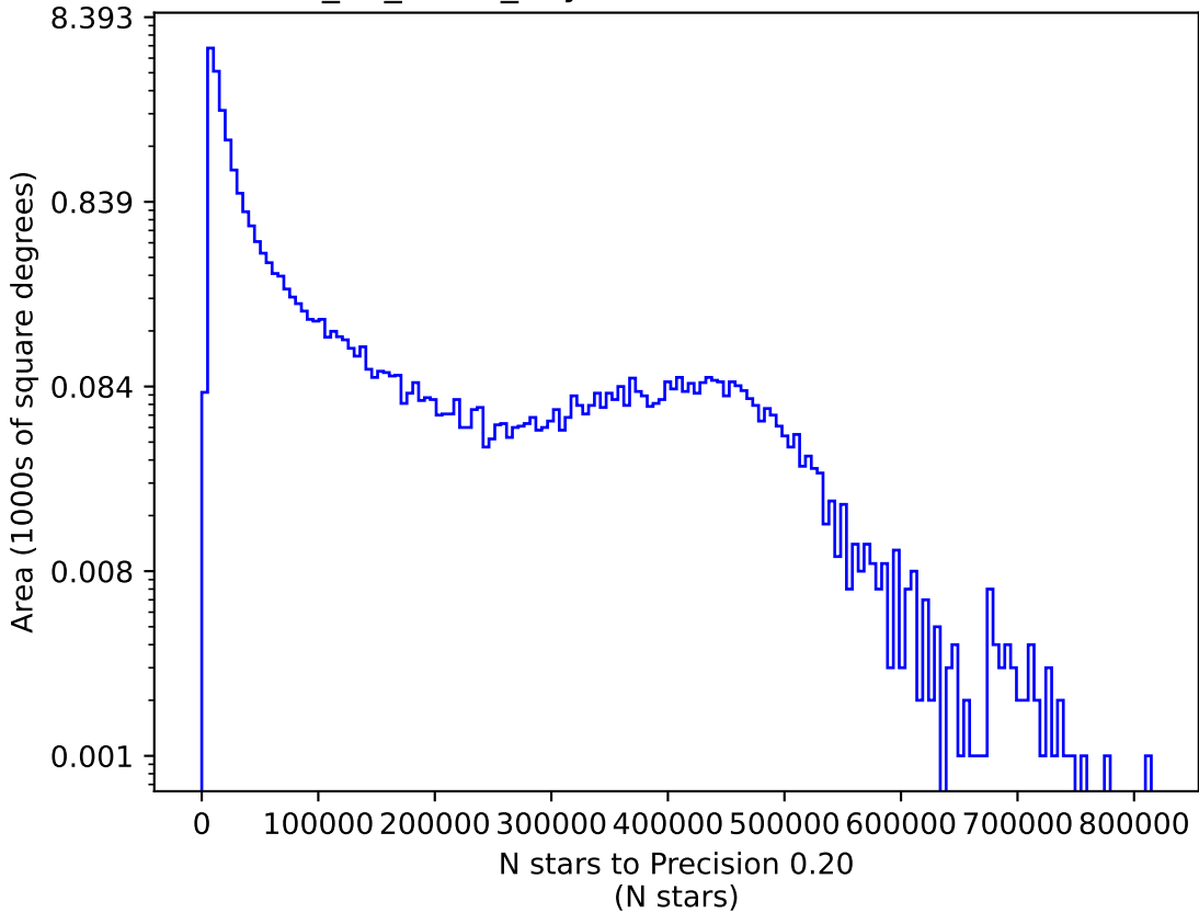
too_10_4v3.4_10yrs i: N stars to Precision 0.20
