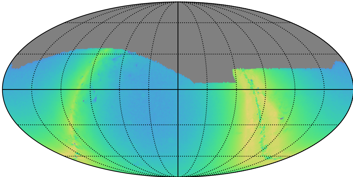
too_10_4v3.4_10yrs g: N stars to Precision 0.20
