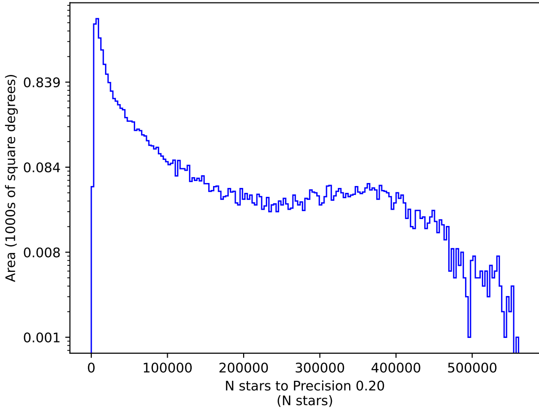
too_10_4v3.4_10yrs g: N stars to Precision 0.20
