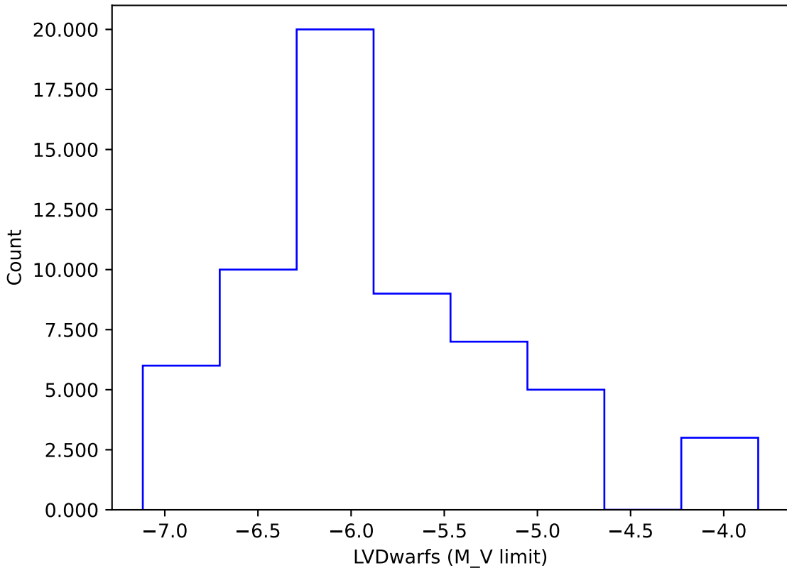
too_10_4v3.4_10yrs gi: LVDwarfs
