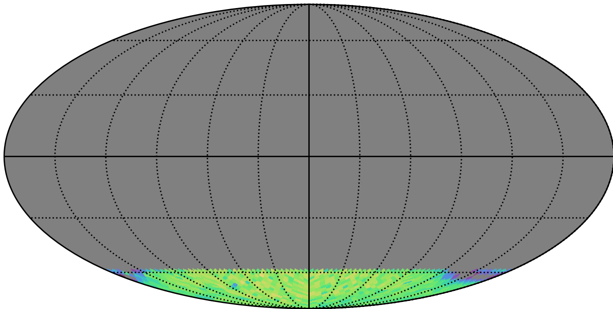
too_10_4v3.4_10yrs gi SCP: LVDwarfs
