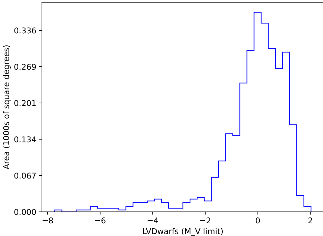
too_10_4v3.4_10yrs gi SCP: LVDwarfs
