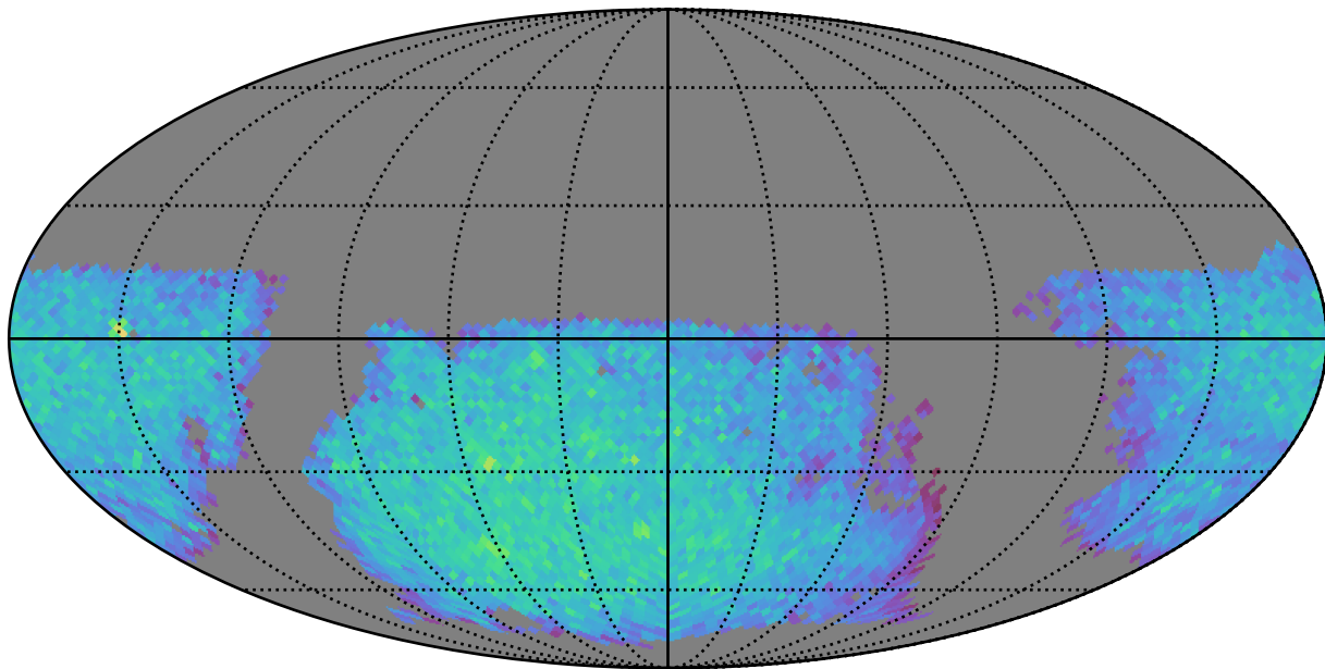
too_10_4v3.4_10yrs gi: LVDwarfs
