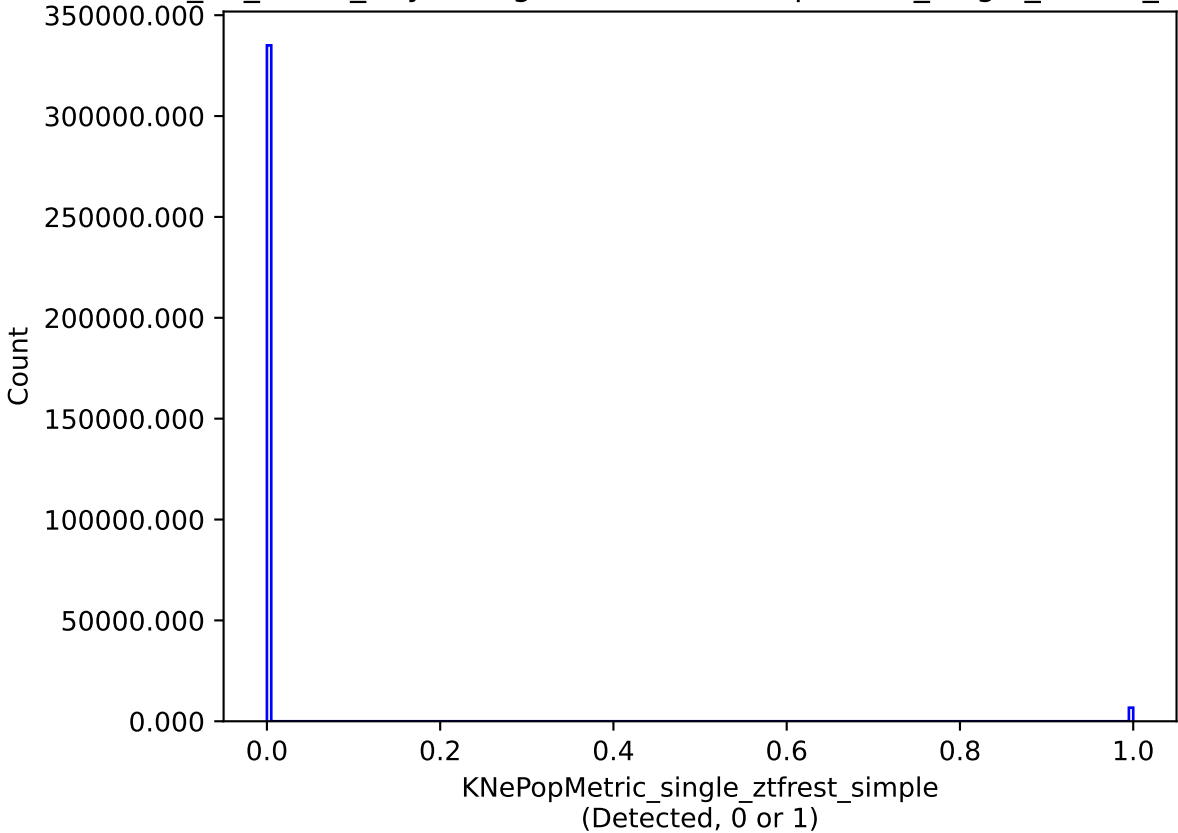
too_10_4v3.4_10yrs single model: KNePopMetric_single_ztfrest_simple
