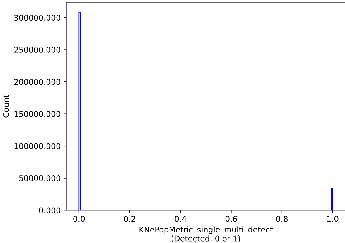
too_10_4v3.4_10yrs single model: KNePopMetric_single_multi_detect
