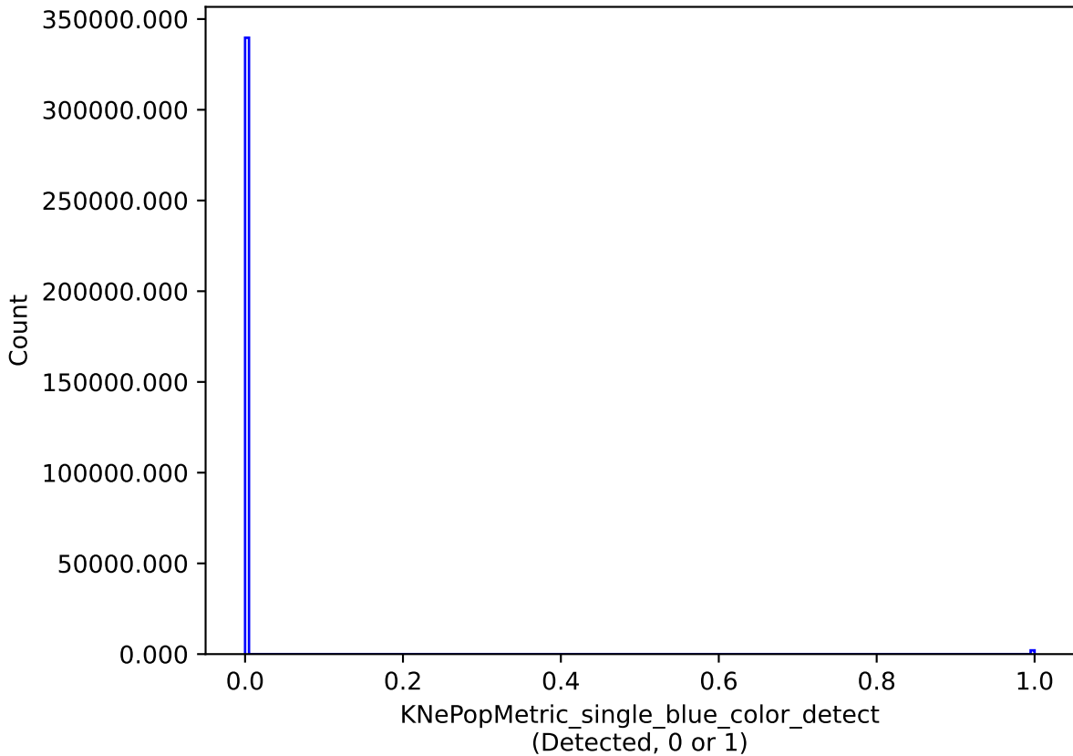
too_10_4v3.4_10yrs single model: KNePopMetric_single_blue_color_detect
