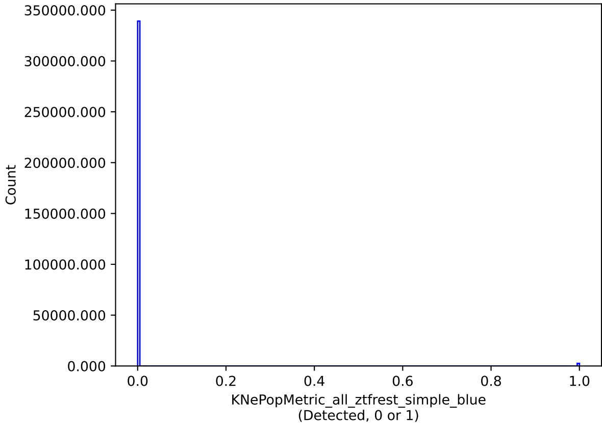
too_10_4v3.4_10yrs all models: KNePopMetric_all_ztfrest_simple_blue
