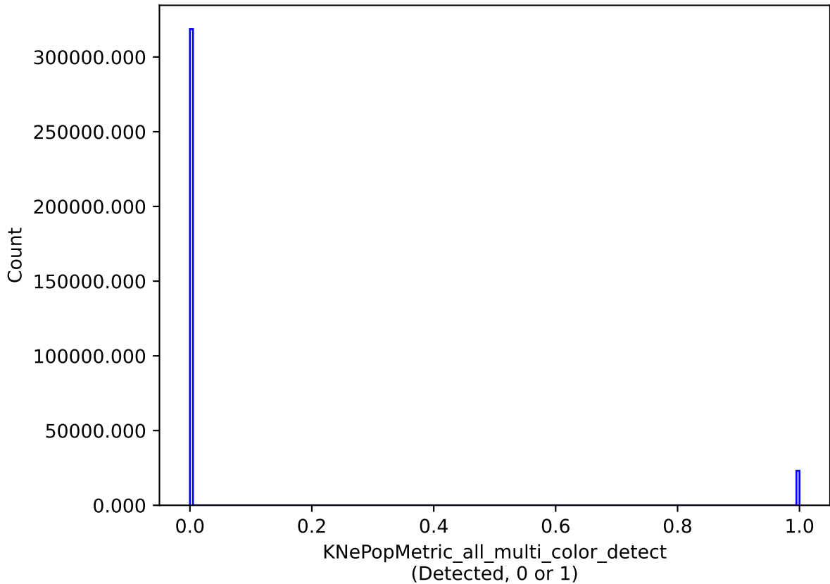
too_10_4v3.4_10yrs all models: KNePopMetric_all_multi_color_detect
