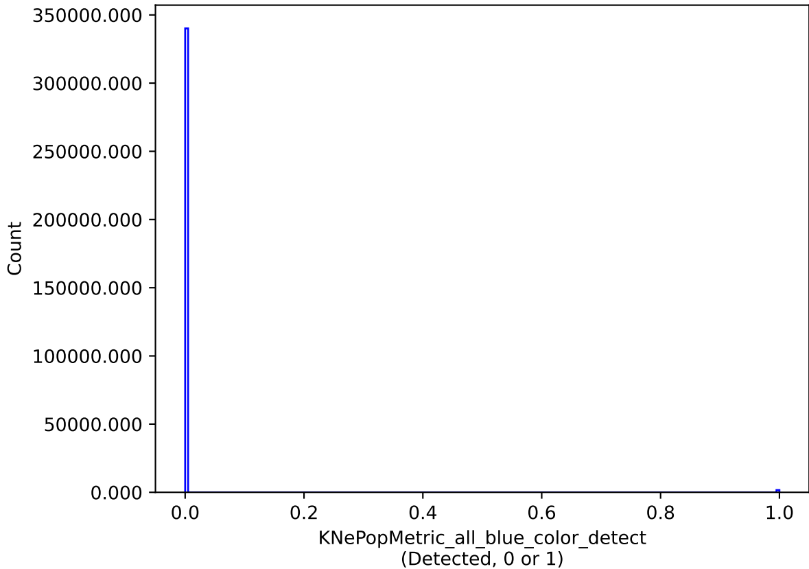
too_10_4v3.4_10yrs all models: KNePopMetric_all_blue_color_detect
