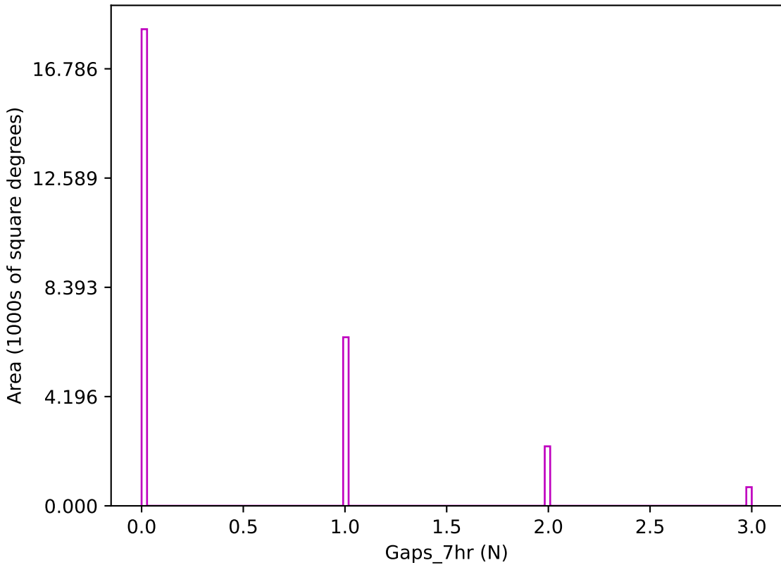
too_10_4v3.4_10yrs z band: Gaps_7hr
