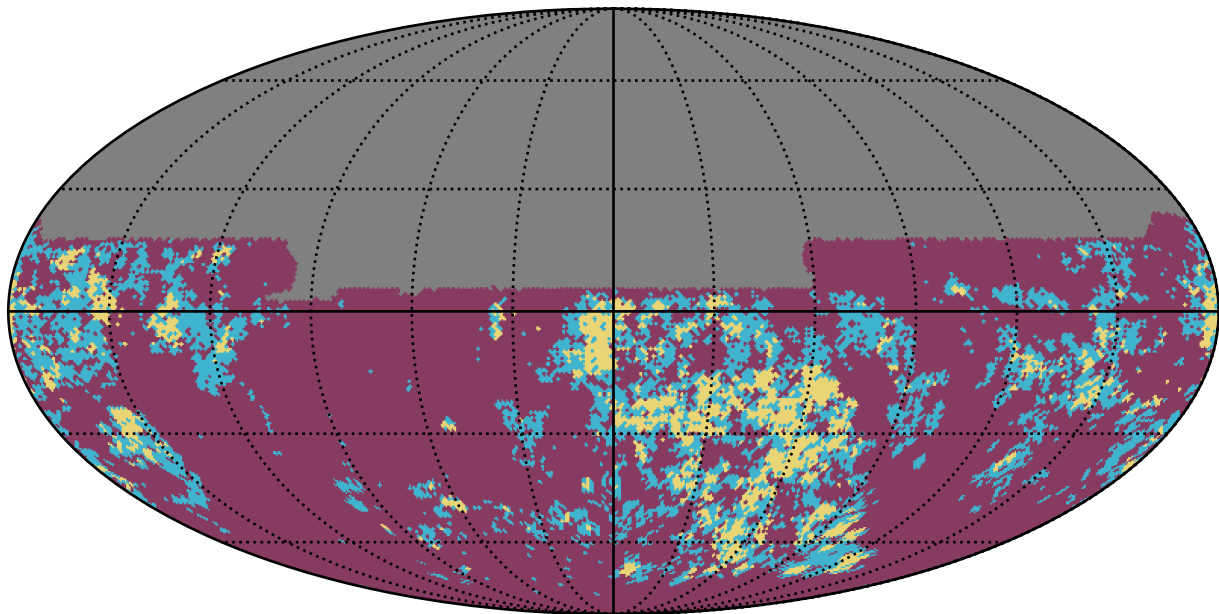
too_10_4v3.4_10yrs y band: Gaps_7hr
