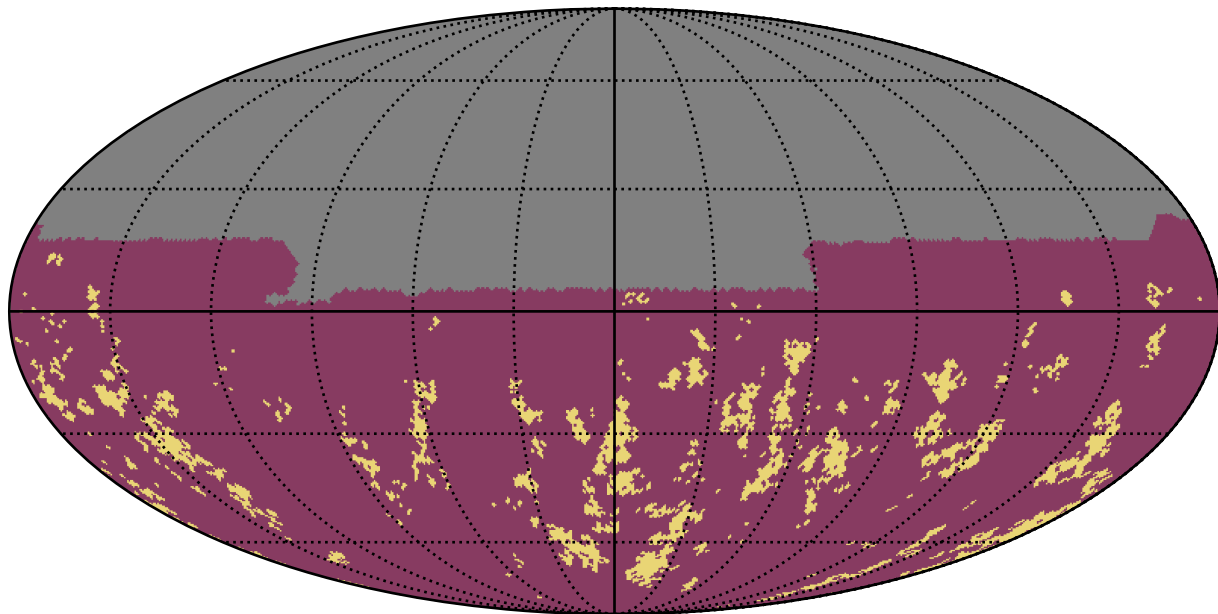
too_10_4v3.4_10yrs u band: Gaps_7hr
