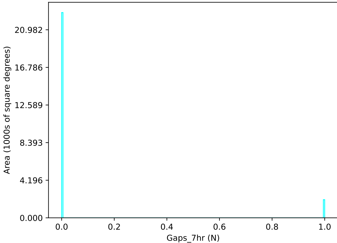
too_10_4v3.4_10yrs u band: Gaps_7hr
