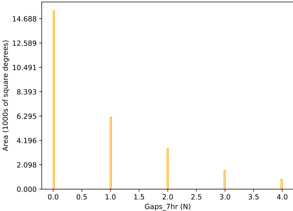
too_10_4v3.4_10yrs r band: Gaps_7hr
