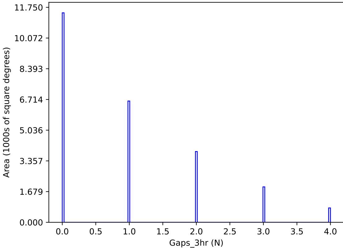
too_10_4v3.4_10yrs y band: Gaps_3hr
