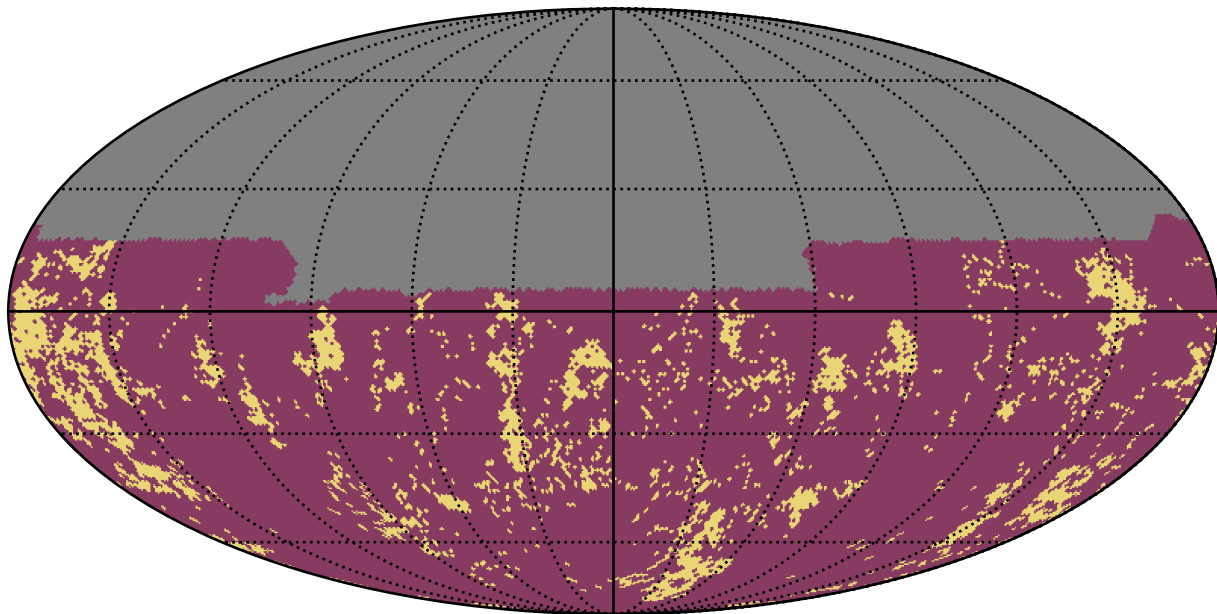
too_10_4v3.4_10yrs u band: Gaps_3hr
