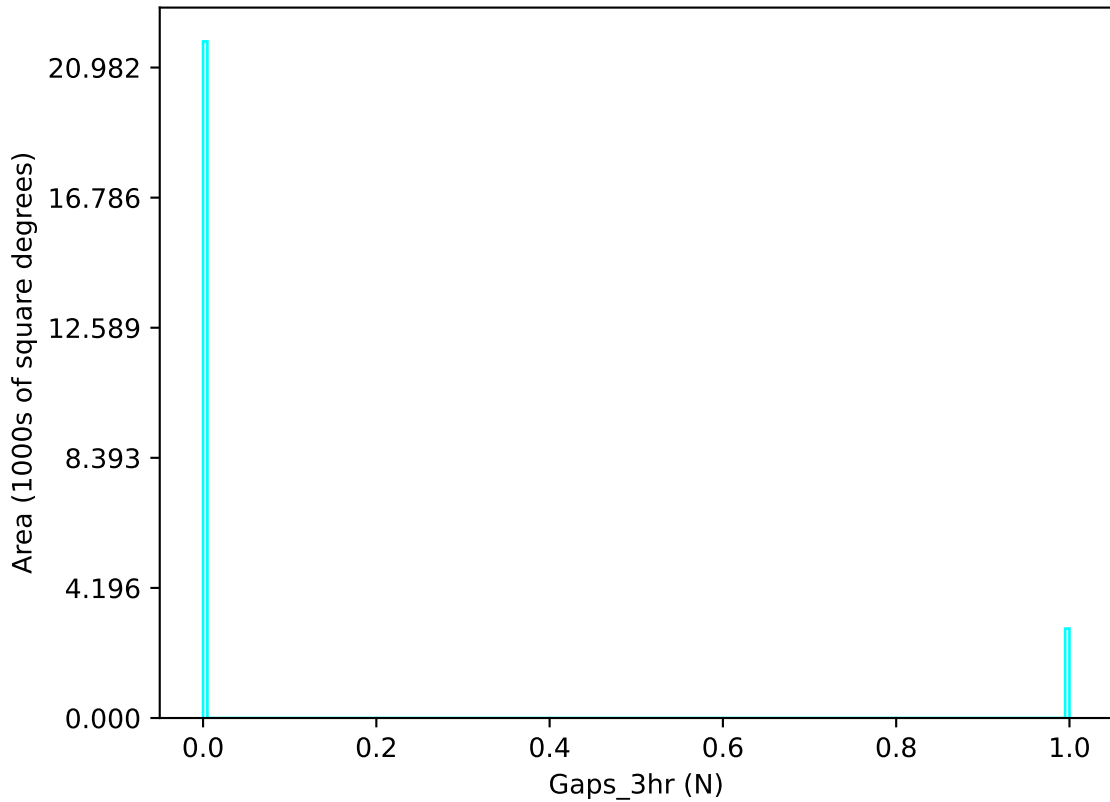
too_10_4v3.4_10yrs u band: Gaps_3hr
