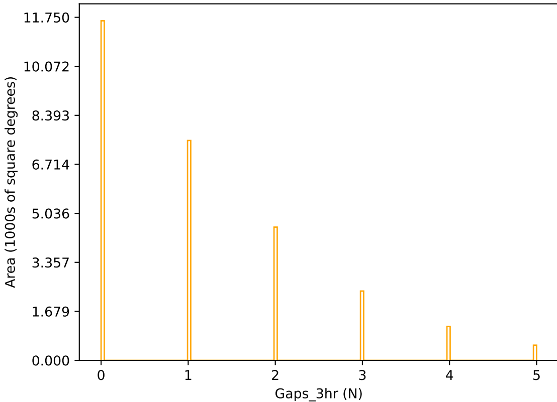
too_10_4v3.4_10yrs r band: Gaps_3hr
