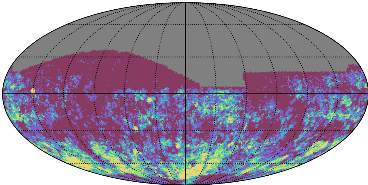
too_10_4v3.4_10yrs i band: Gaps_3hr
