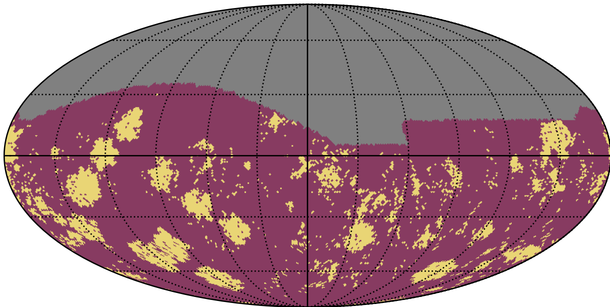
too_10_4v3.4_10yrs g band: Gaps_3hr
