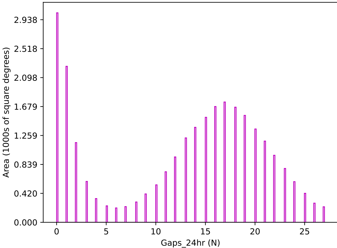
too_10_4v3.4_10yrs z band: Gaps_24hr
