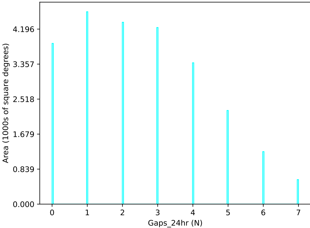
too_10_4v3.4_10yrs u band: Gaps_24hr
