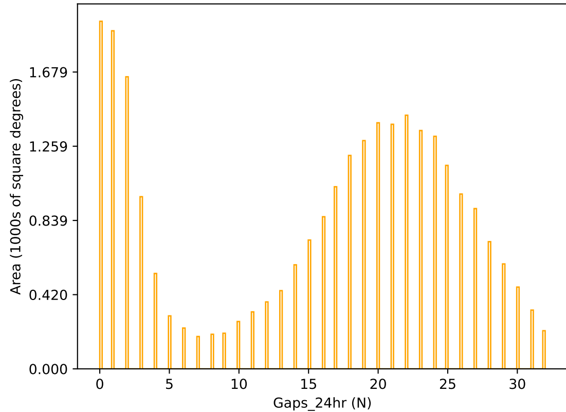
too_10_4v3.4_10yrs r band: Gaps_24hr
