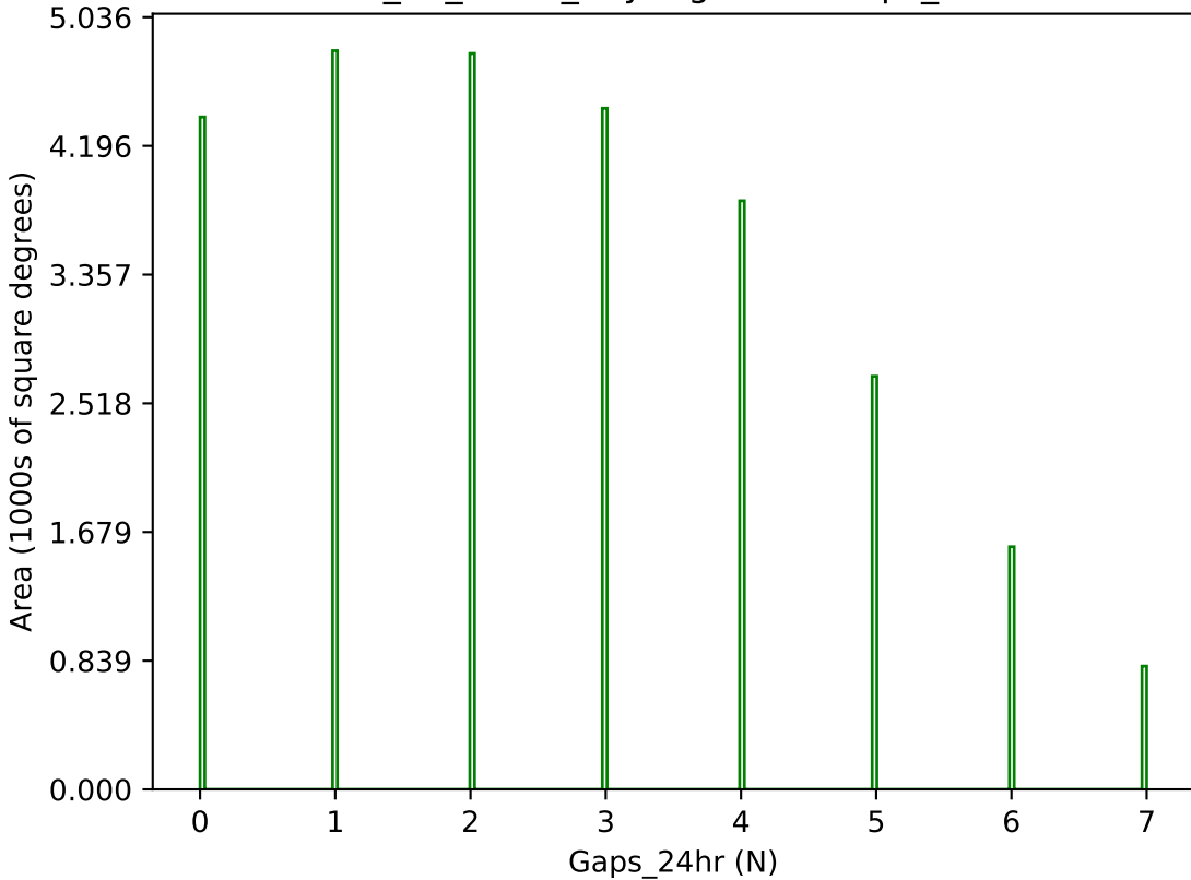
too_10_4v3.4_10yrs g band: Gaps_24hr
