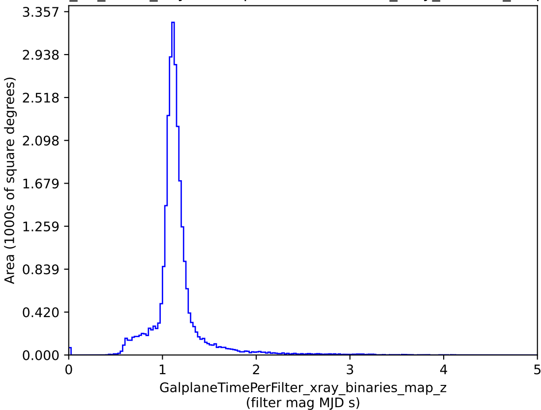
too_10_4v3.4_10yrs : GalplaneTimePerFilter_xray_binaries_map_z
