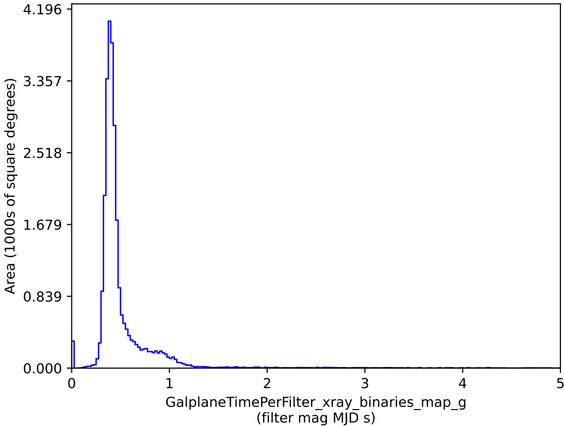
too_10_4v3.4_10yrs : GalplaneTimePerFilter_xray_binaries_map_g
