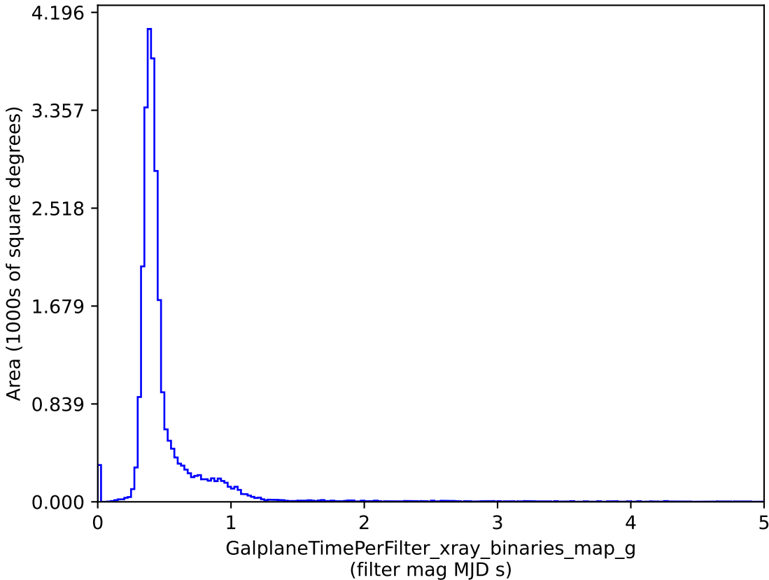
too_10_4v3.4_10yrs : GalplaneTimePerFilter_xray_binaries_map_g
