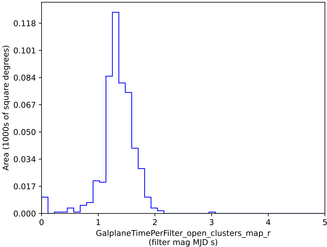
too_10_4v3.4_10yrs : GalplaneTimePerFilter_open_clusters_map_r
