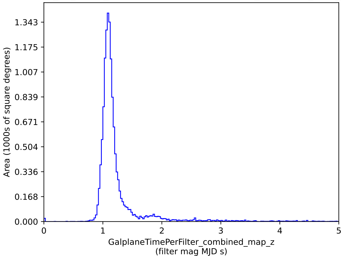
too_10_4v3.4_10yrs : GalplaneTimePerFilter_combined_map_z
