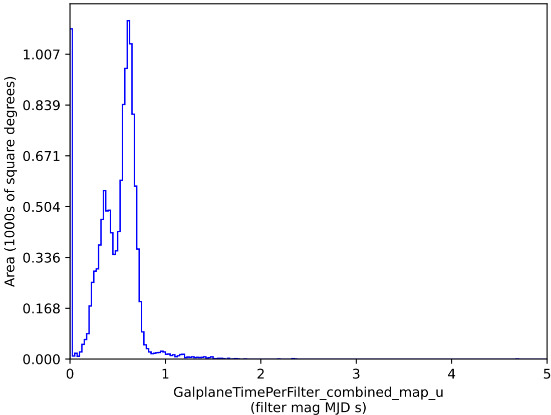
too_10_4v3.4_10yrs : GalplaneTimePerFilter_combined_map_u
